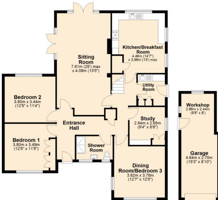
Ground Floor Approx. 146.7 sq. metres (1579.1 sq. feet)
