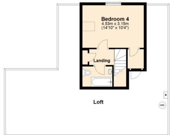
First Floor Approx. 25.6 sq. metres (275.2 sq. feet)
