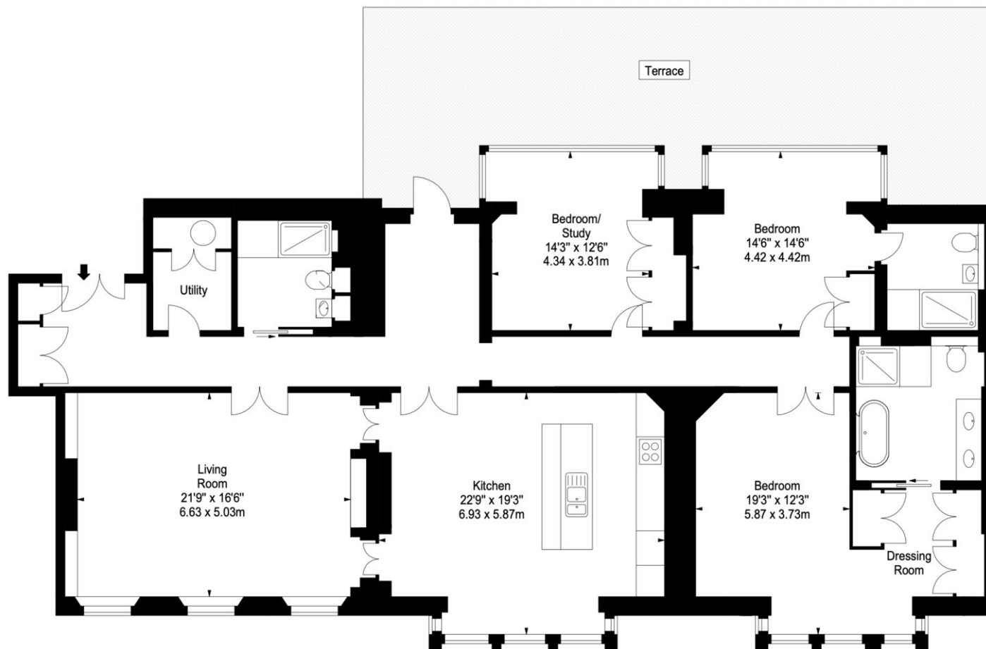
FIRST FLOOR
