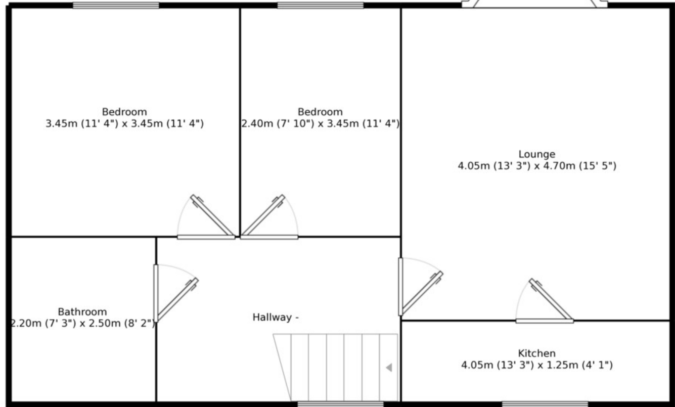
First Floor Floor Size: 58.9 m 2 , 634.0 ft 2
