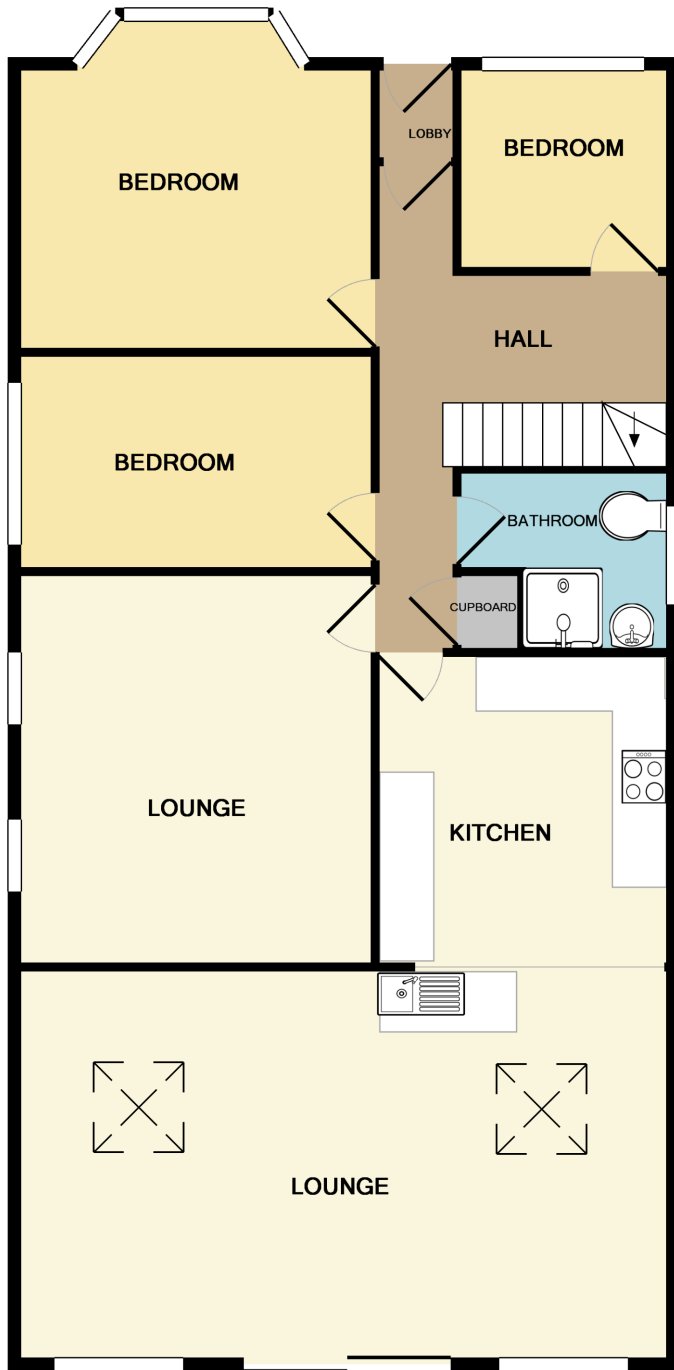
GROUND FLOOR APPROX. FLOOR AREA 1153 SQ.FT. (107.1 SQ.M.)
