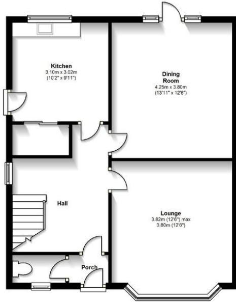
Ground Floor Approx. 57.5 sq. metres (618.5 sq. feet)
