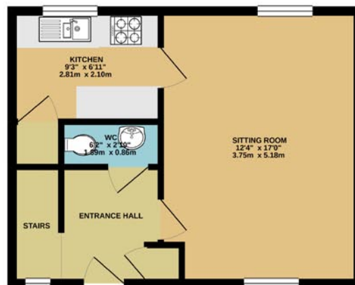
GROUND FLOOR 366 sq.ft. (34.0 sq.m.) approx.
