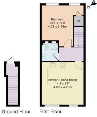
Floor Plan
