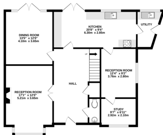
GROUND FLOOR 1035 sq.ft. (96.2 sq.m.) approx.
