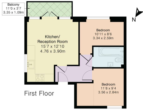
Floor Plan
