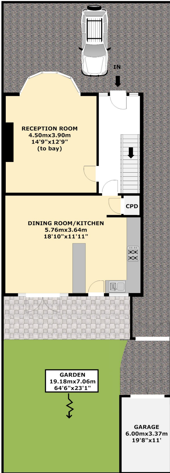
GROUND FLOOR
