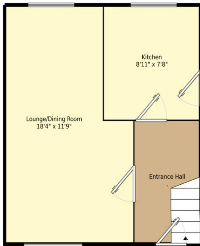
Ground Floor Floor Size: 30.5 m 2 , 328.5 ft 2
