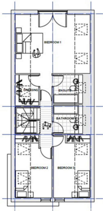
FIRST FLOOR 1:100
