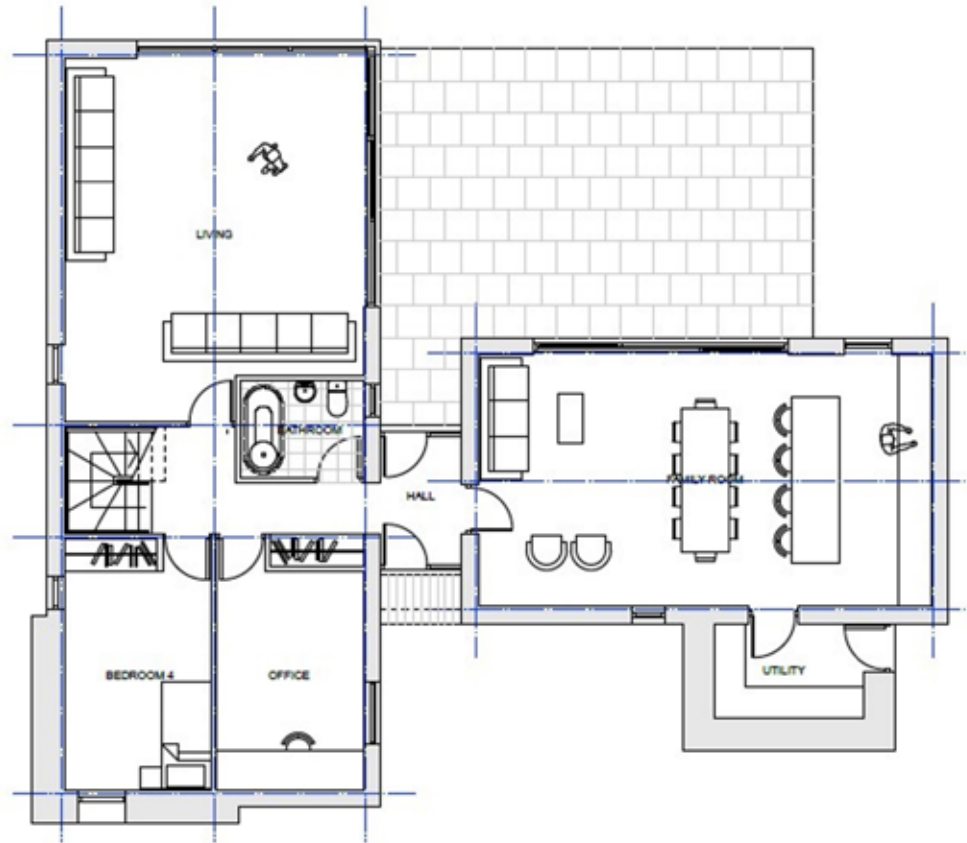
GROUND FLOOR 1:100
