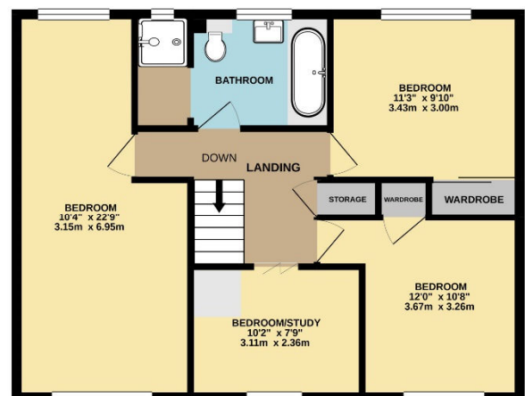
1ST FLOOR 680 sq.ft. (63.2 sq.m.) approx.
